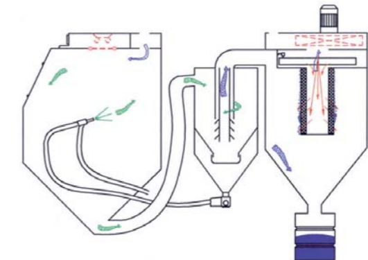
Injector principle
