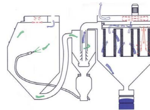
Pressureblasting principle
